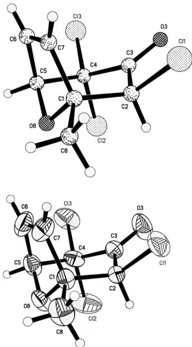
Figure 1. X-ray structure of (2- endo )-2,4,4-trichloro-1-methyl-8-oxabicyclo[3.2.1]oct-6-en-3-one ( 7bn ); see also ref. [9]
