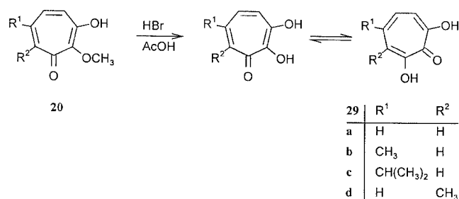
Scheme 6. Demethylation of 3-hydroxy-2-methoxytropone 20
