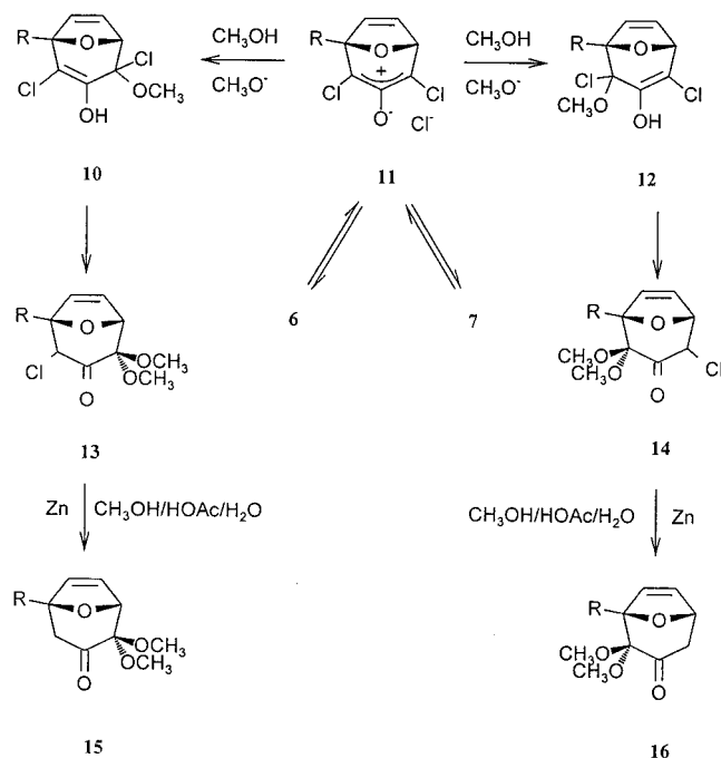
Scheme 2. Methanolysis and dechlorination of trichloro-8-oxabicyclo[3.2.1]oct-6-en-3-ones 6 , 7
