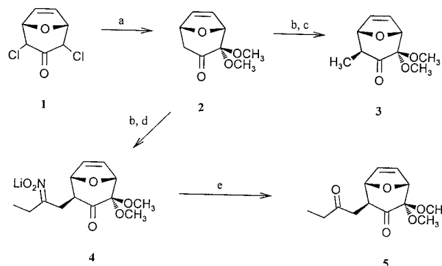
Scheme 1. Formation and alkylation of 2 : a) \text{CH}_3\text{ONa}/\text{CH}_3\text{OH} , 38%; b) LDA, THF; c) \text{CH}_3\text{I} , HMPA, 82%; d) 2-nitrobut-1-ene; e) 3 M \text{H}_2\text{SO}_4 , \text{H}_2\text{O}/\text{CH}_3\text{OH} , 64%
