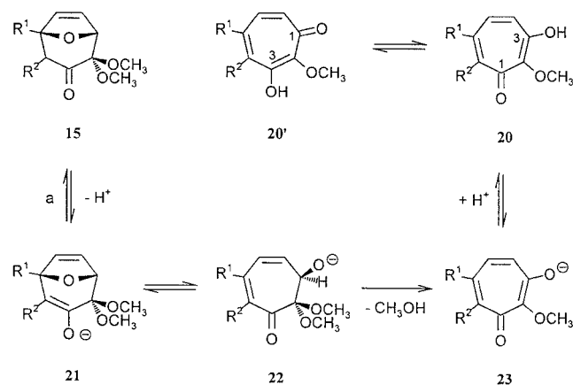
Scheme 4. Cleavage of oxabicyclic oxo acetals 15 : a) KOH, \text{CH}_3\text{OH} , 65^\circ\text{C}
