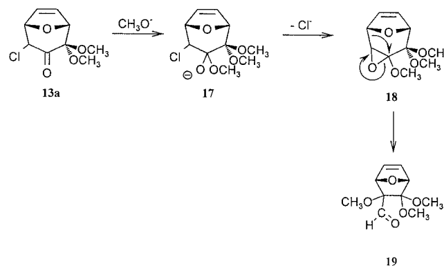
Scheme 3. Proposed rearrangement mechanism of the chloro acetal 13a
